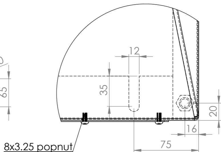
DETAIL C SCALE 2 : 5
